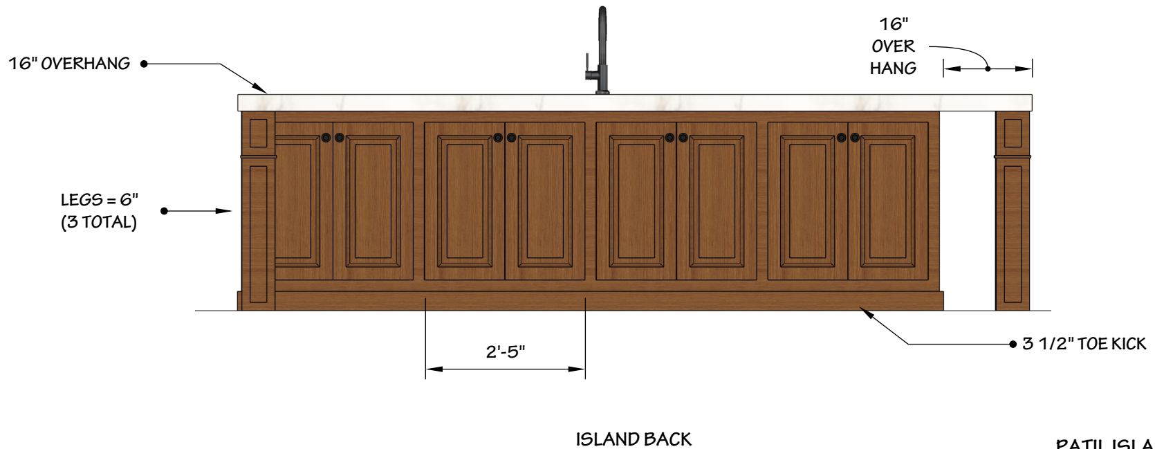
PATIL ISLAND ELEVATIONS SCALE: 1/2" = 1'-0"
